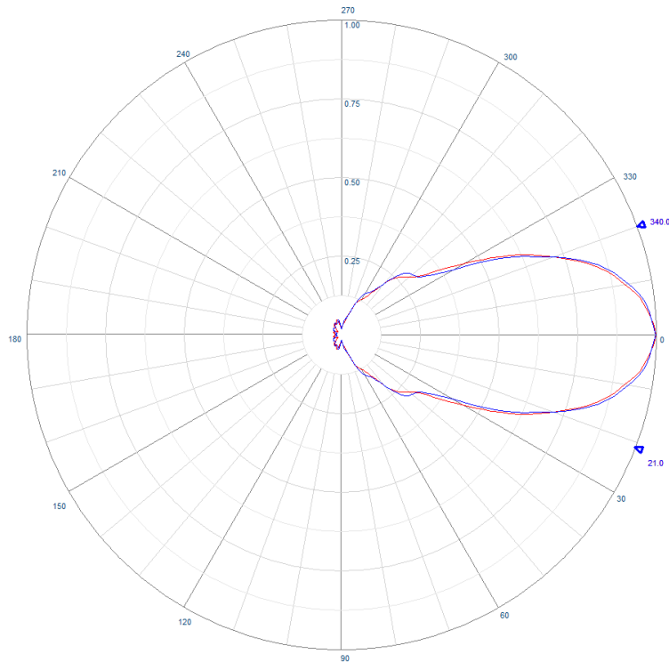
Example Polar radiation pattern - Y615TV-SS-RCM
