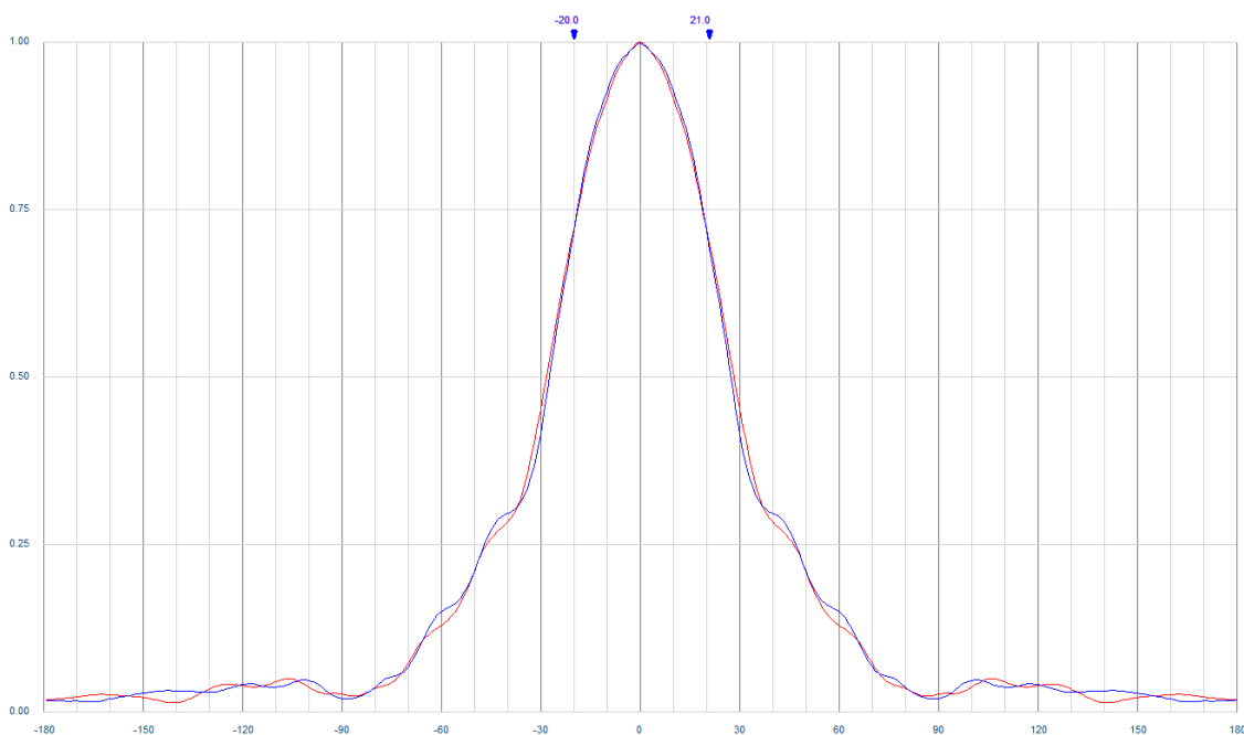
Example Cartesian radiation pattern - Y615TV-SS-RCM
