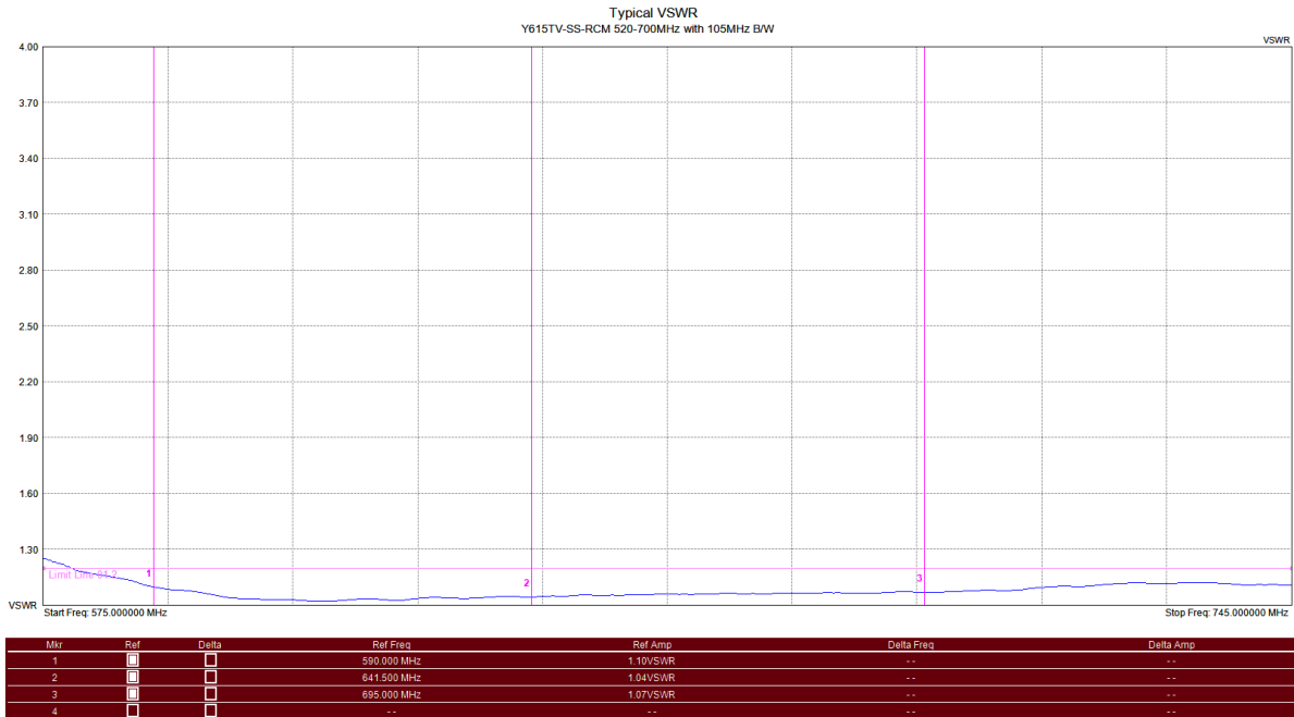
Typical VSWR - Y615TV-SS-RCM
